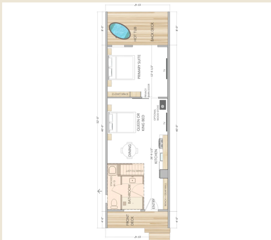
Floor plan: Sierra
