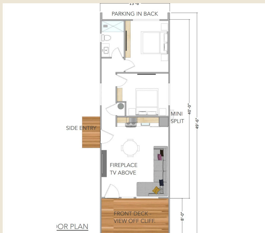
Floor plan: Gallatin II
